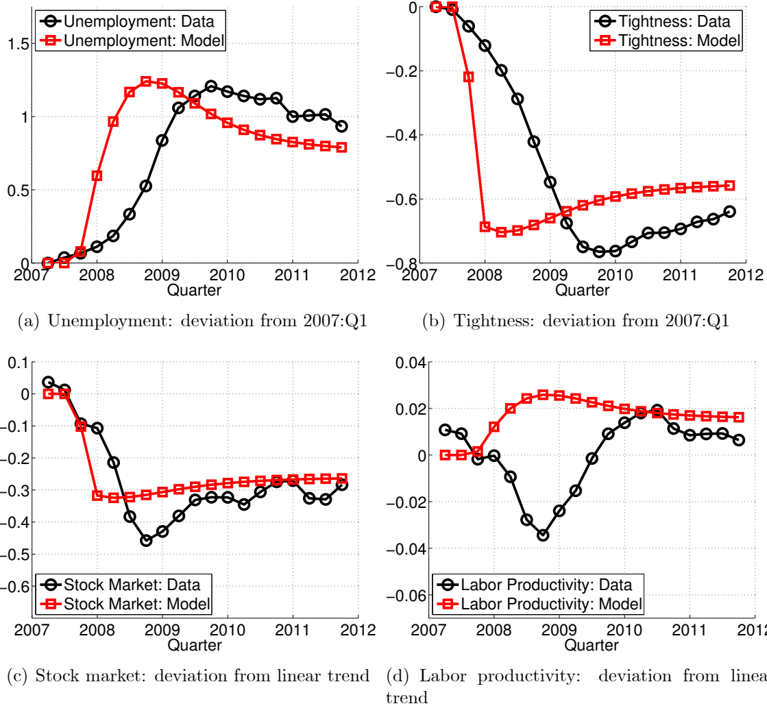
Figure 7: Impulse response to a negative sentiment shock
